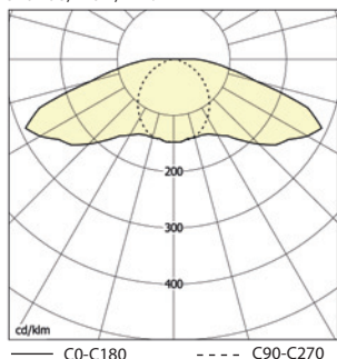
SKOPOS, 1x8W, IP 40
