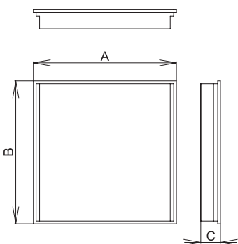
BARBET-T5-BAP-DL, 4x14W, IP20
